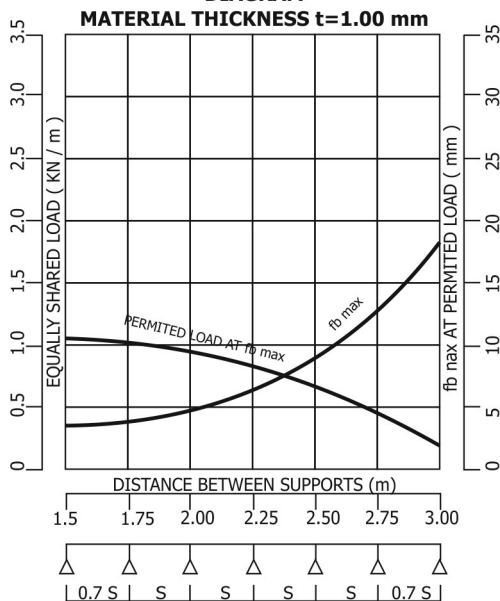
CABLE TRAY H:35 LOADING DIAGRAM
